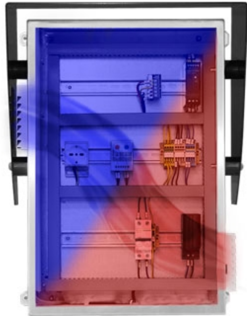
Automatic temperature regulation system with ventilation fan and internal heating unit.
